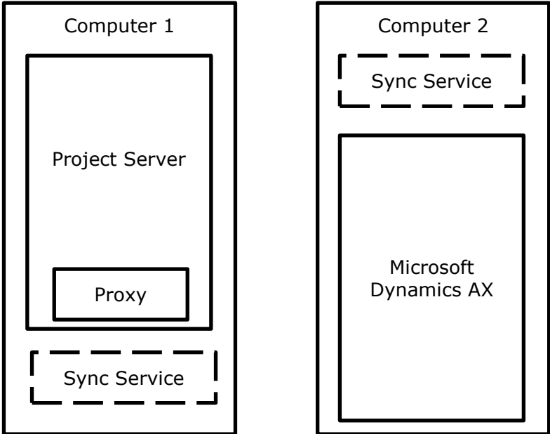
Figure 3: Two-server topology
